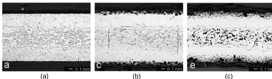
Figure 3. Image of the cross-section of the fuel plate submitted to \sim 450 W/cm 2 (a); \sim 500 W/cm 2 (b); and \sim 550 W/cm 2 (c) from Leenaers' work [22], showing granular aspect of pitting corrosion on the Al5754 alloy cladding.
