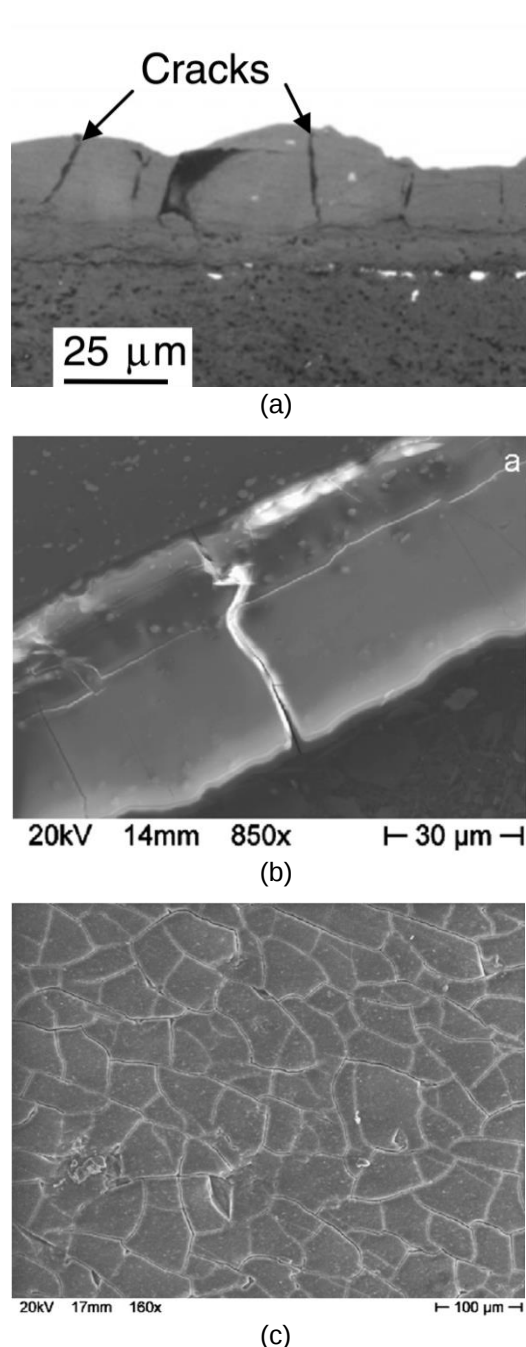
Figure 4. Micrograph showing cracks in the oxide layer of fuel cladding: AG3NE cladding in SIMONE LC-04 fuel test [21] (a), and; AlFeNi cladding from U_3Si_2 fuel [23] cross section (b) and surface (c).
