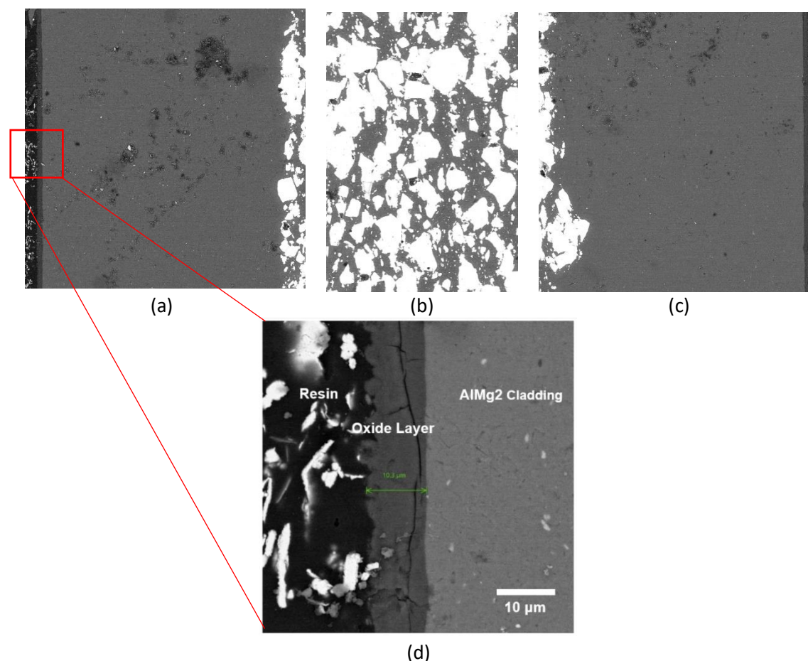
Figure 2. Backscatter electron SEM Image of the irradiated fuel plate over the width (cross-section), showing overview of the fuel cross-section (a-c); and more detailed micrograph of the oxide layer on the fuel cladding (d).
