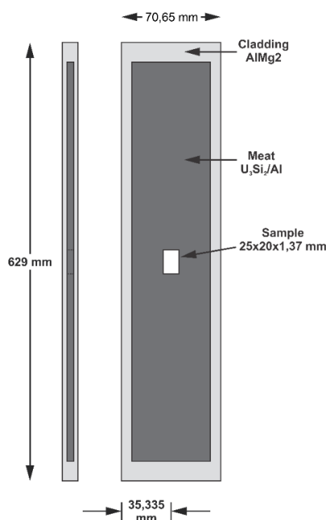
Figure 1. Sampling position in CBBJ251 fuel plate using punching-device. The dimension of the fuel plate was based on non-destructive test result [24].
