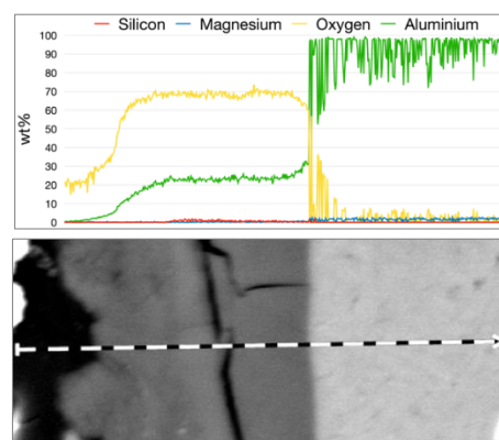
Figure 5. Semi-quantitative linescan covering the AlMg2 cladding and the oxide layer.
