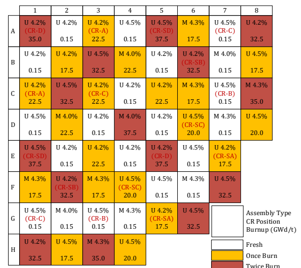
Figure 1. Quarter-core geometry [10].
