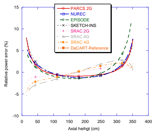
Figure 8. Axial power distribution relative error.
