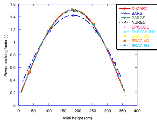
Figure 7. Axial power distribution for HZP condition.
