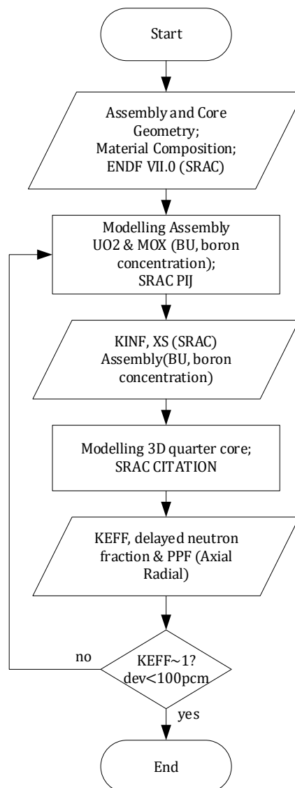
Figure 2. Calculation flowchart.
