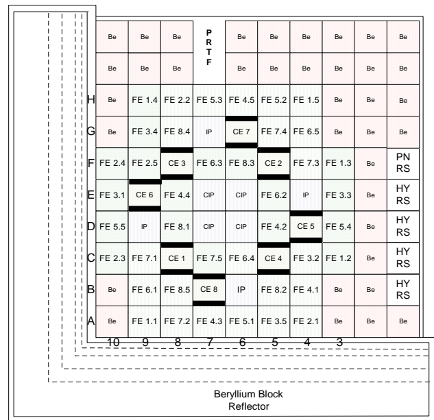
Fig. 1. Core configuration of RSG-GAS[16]
