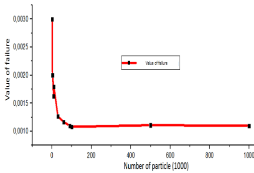
Figure 9. Graph of value of failure for number of particles of HTR-PM.
