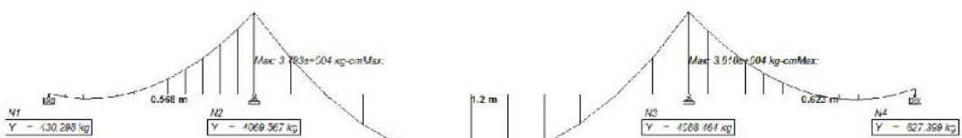
BENDING MOMENT
