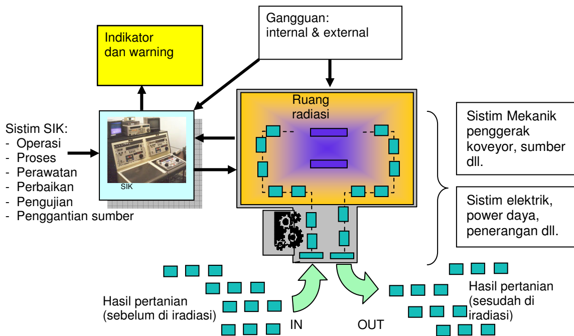
Gambar 6. Disain konsep instalasi irradiator gamma ISG-500 [13] .
