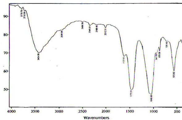
Figure 7. FTIR Spectrum of HA powder.
