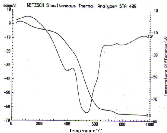
Gambar 2. DTA-TG curve of the white gel dried at 340°C.
