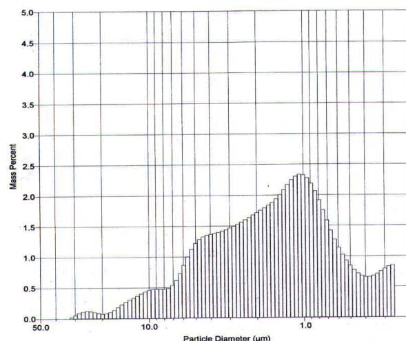
Figure 6. Particle distribution of HA powder
