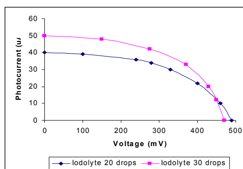
Figure 7. I-V characteristics of two solar cell devices, with Iodolyte (a) 20 drops and (b) 30 drops.
