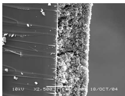
Figure 4. Cross-section of TiO 2 film on glass substrate
