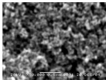
Figure 3. SEM picture of nanoporous TiO 2 film
