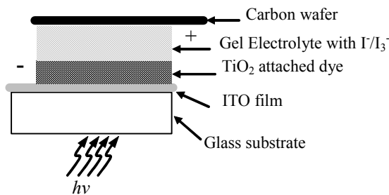
Figure 2. Structure of dye-sensitized solar cell
