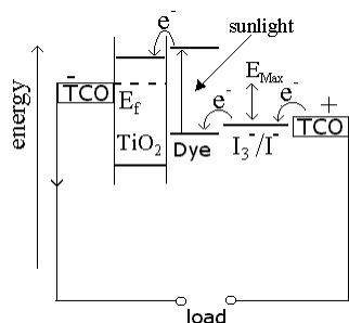
Figure 1. Principle of dye sensitized solar cell
