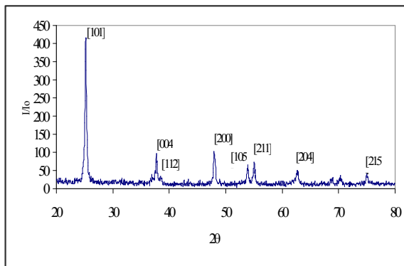
Figure 5. XRD pattern of TiO 2 film
