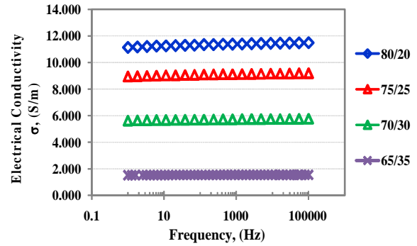
Figure 4. Electrical conductivity of composite material in the varying compositions
