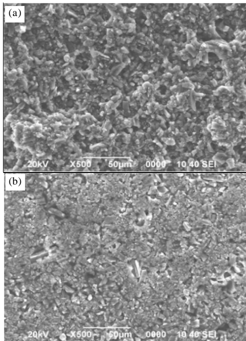
Figure 2. GDL sheet morphology with composition for carbon: polymer = 80:20, (a). The upper surface and (b). Bottom.
