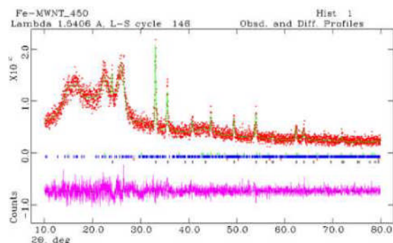
Figure 2. Refinement patterns of XRD data of Fe 2 O 3 -MWCNT (450 °C)
