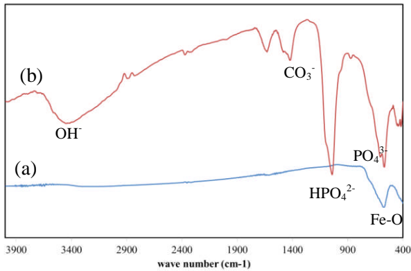
Figure 5. Infra red spectra of magnetite nanoparticle (a) and K50 composite (b).
