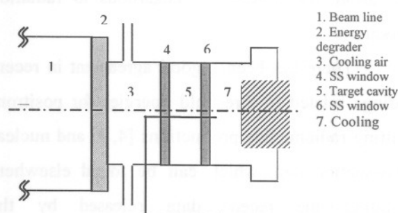
Fig. 1 Schematic design of the Liquid Target Chamber for ^{18}\text{F} Production at the Cyclotron Division of Centre for Radioisotopes and Radiopharmaceuticals.
