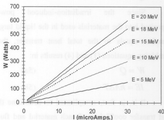
Fig. 2 Power (W) deposited into a water target as a function of proton beam current (I) for several proton energies.
