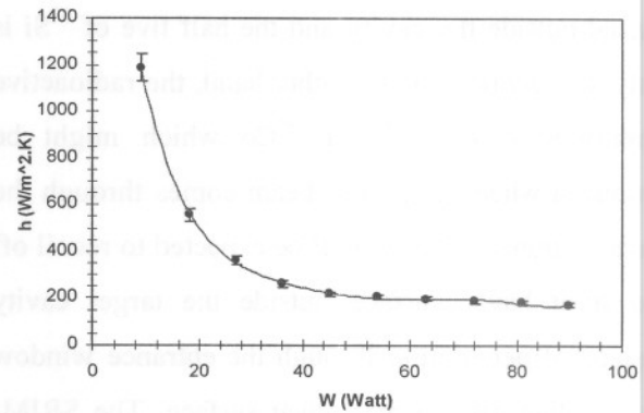
Fig. 3 Overall heat transfer coefficient ( h ) as a function of power ( W ) deposited into the water target.
