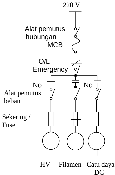
Gambar 2. Diagram system tenaga Pesawat sinar-X Fluoroscopy (3)
