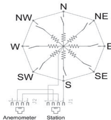
Gambar 4. Rangkaian Sensor Arah Angin [3]
